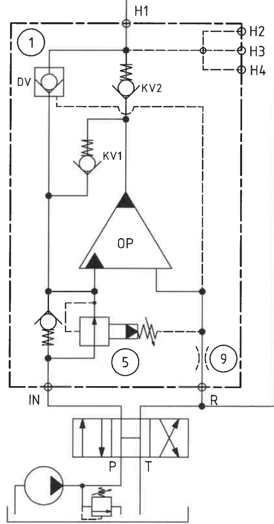
Assembly Drawing: 2-128-0__
