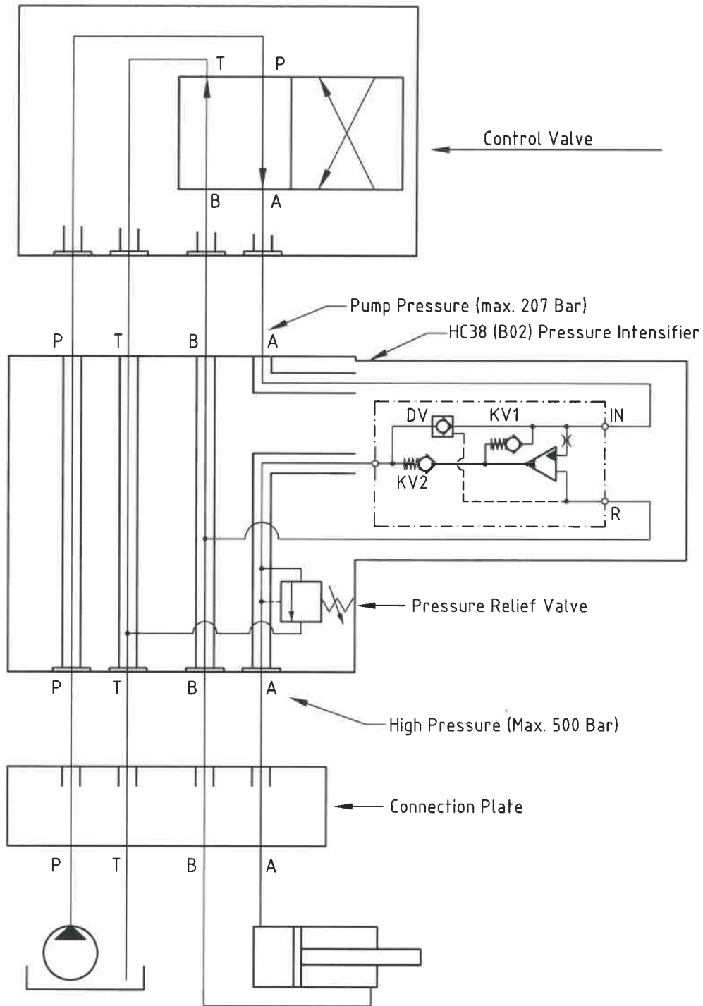
Assembly Drawing: 3-217-0__
