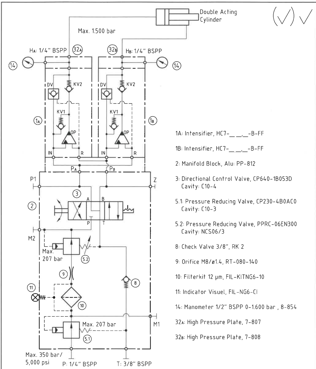
Assembly Drawing: M-HC7-812A-1002DA-0_
